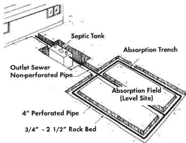
Typical Onsite Wastewater System
